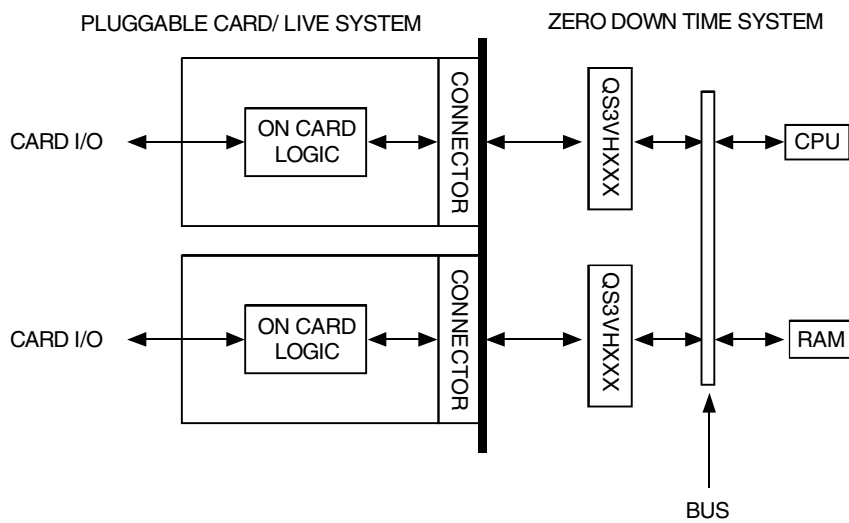
Hot-Swapping
